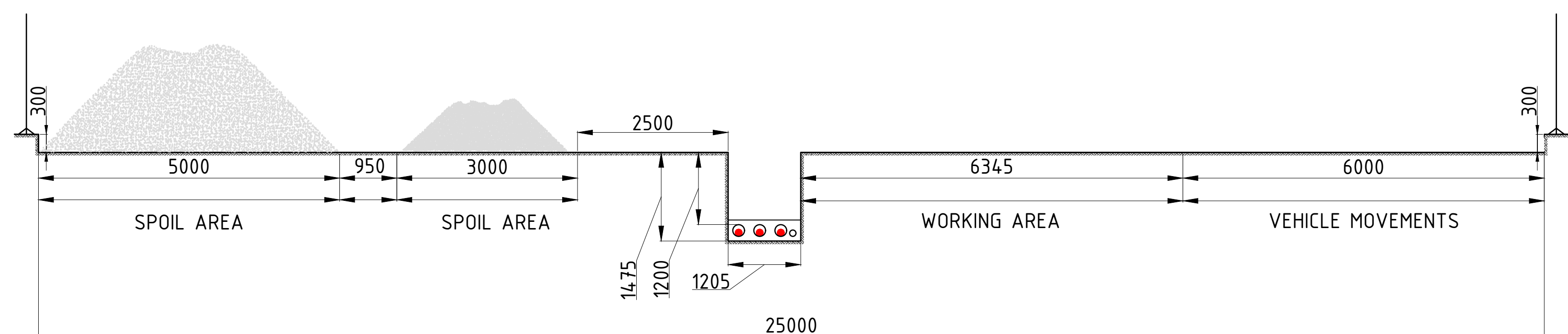
FLAT FORMATION TRENCH CONFIGURATION
